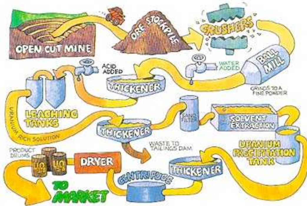
Preparation of yellow cake, purified U_3O_8(s) (Courtesy of the Uranium Information Center)
